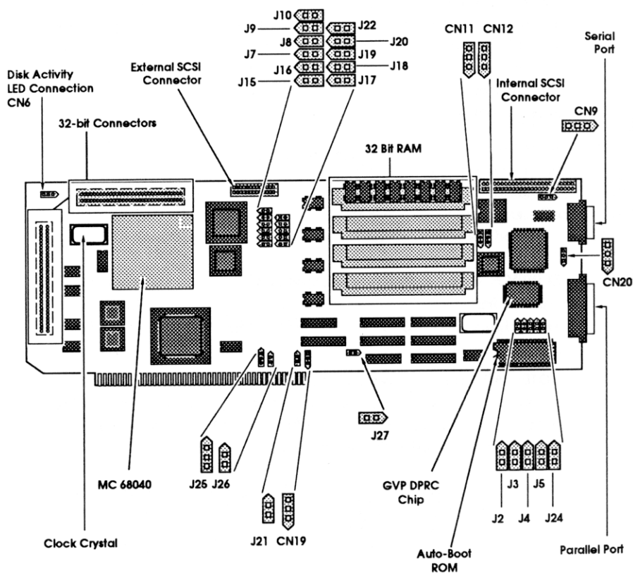
Figure 3.3 – A2000 G-Force '040 board showing jumper locations.
