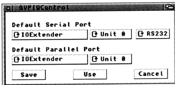
Figure 7.1 – GVPIOControl window.
