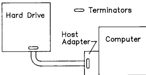
Fig. 6 - Standard System Termination
